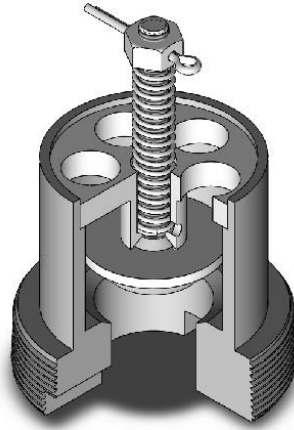
Figure 1: Valve Cutaway
